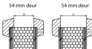
Glaslatten Fire Proof 60
