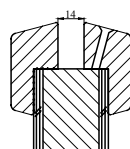
Glaslatten Fire Proof 30
