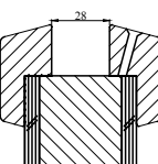
Glaslatten Fire Proof 30
